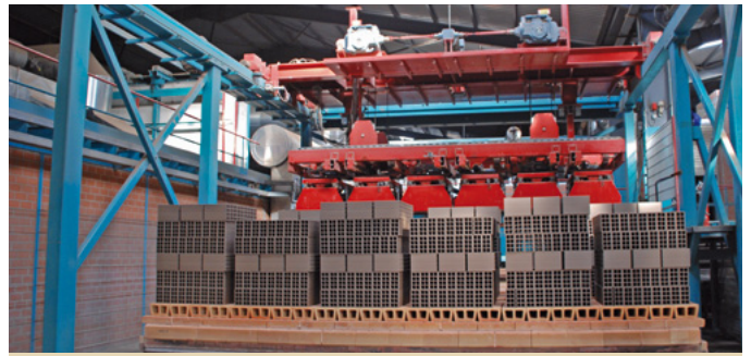
Installation d'empilage, usine 2 Setting installation, plant 2
